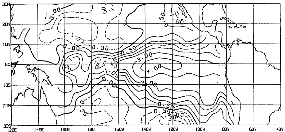
Fig. 1. SST anomalies (°C) during winter 1982-83.
