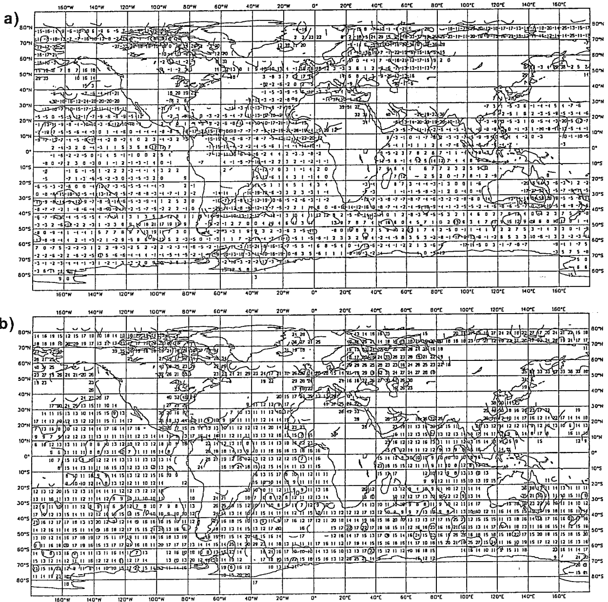
Fig. A1 (a) is bias of stability index (S) for NOAA-9 Clear Soundings, February 87. (Bias = observation minus first-guess, averaged over the studied 15-day period in February 1987). (b) is standard deviation. (c) and (d) are like (a) and (b) respectively but for MSU soundings.
