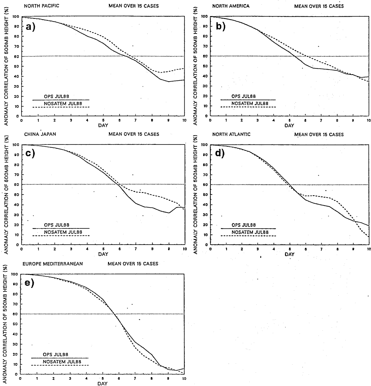
Fig. 3 Anomaly correlation of 500 hPa geopotential height, accumulated on 15 cases for OPS-JUL88 (solid line) and NOSATEM-JUL88 (dashed line) for five limited areas. (a) is for the North Pacific, (b) is North America, (c) is China/Japan, (d) is North Atlantic and (e) is Europe and the Mediterranean.
