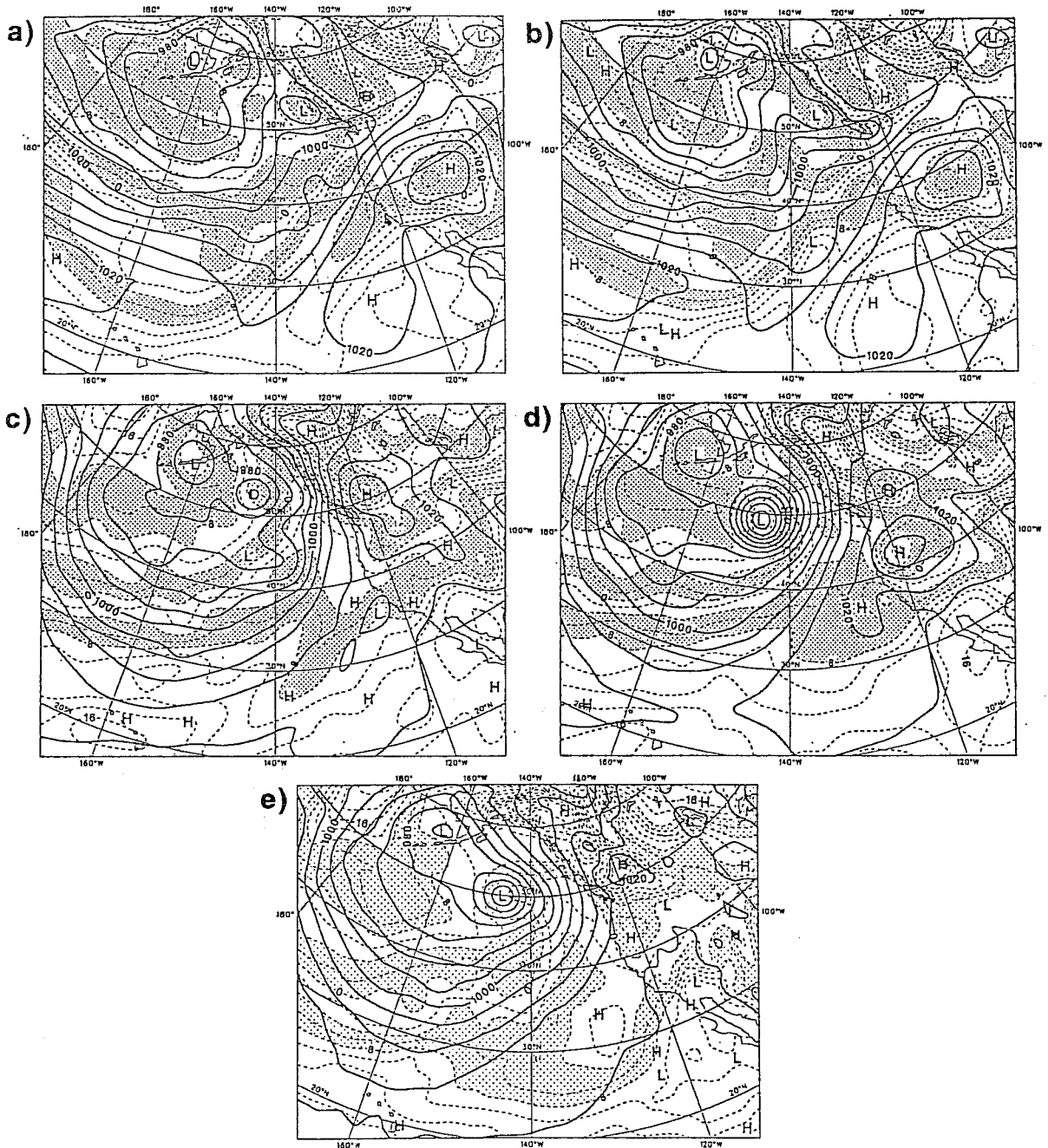
Fig. 5 Mean sea level pressure (hPa, full lines) and 850 hPa temperature (K, dashed lines and shaded in intervals of 4K) in the eastern North Pacific. (a) is the OPS-July 88 analysis at 1 February 1987, 12 UTC and (b) is the corresponding NOSATEM analysis. (c) is the 48-hour forecast from the analysis in (a) and (d) is the corresponding NOSATEM forecast. (e) is the verification analysis for 870203 12 UTC.
