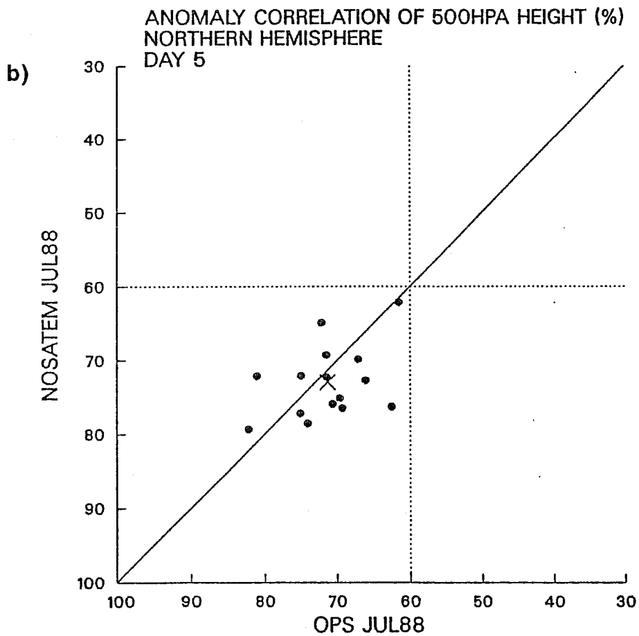
Fig. 2 Scatter diagrams of OPS versus NOSATEM forecast scores for day 5. (a) is with the July-87 system and (b) is with the July-88 system.
