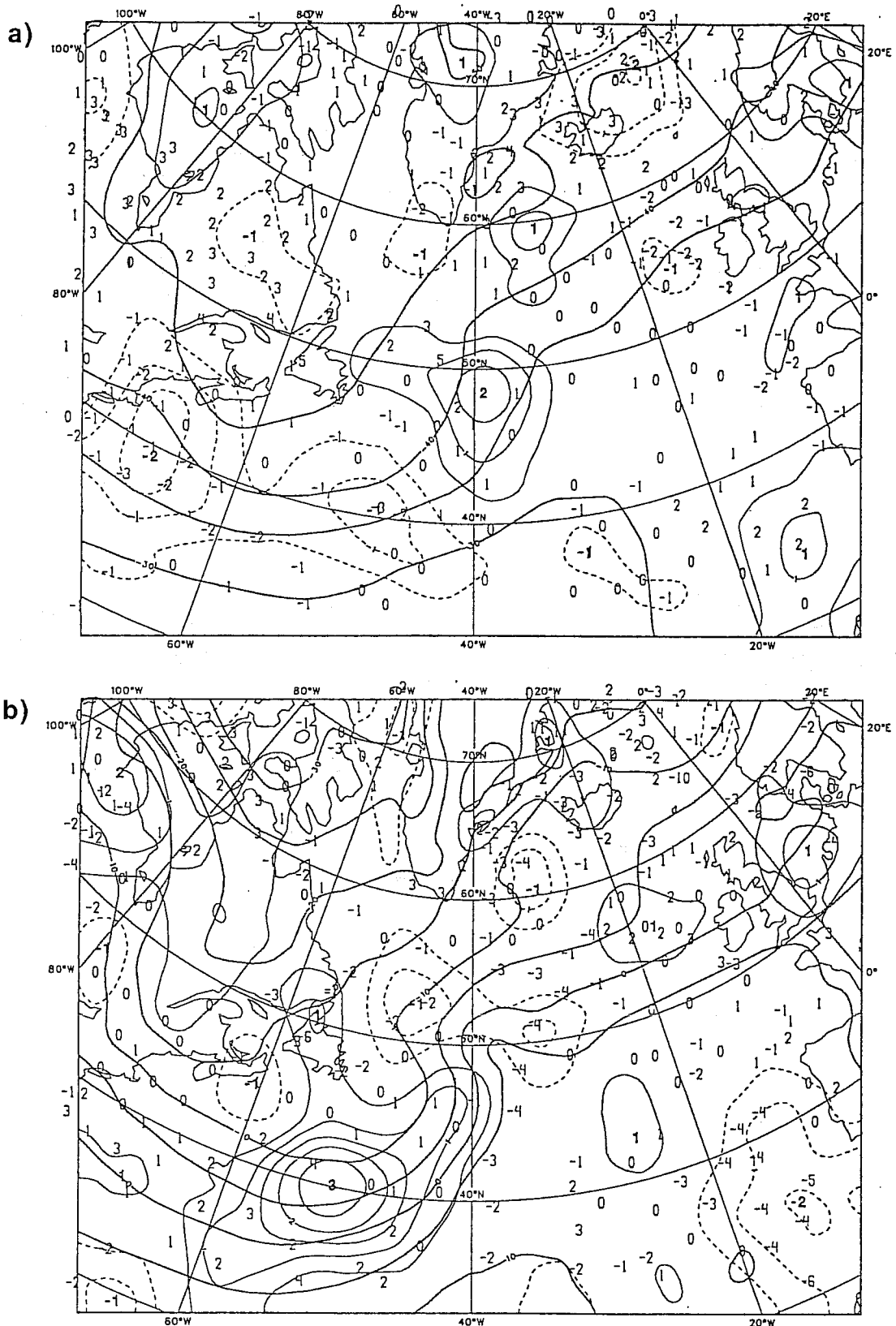
Fig. 6 Observed SATEM layer-mean temperature deviations from first guess in K, 870206-12 UTC, for the North Atlantic. The first-guess field (OPS-JUL88 is contoured with an interval of 5K (solid lines). Also contoured (thin lines) is the analysis increment with an interval of 0.5K : thin full lines are positive (AN-FG) and dashed are negative. (a) is 1000-700 hPa, (b) is 500-300 hPa.
