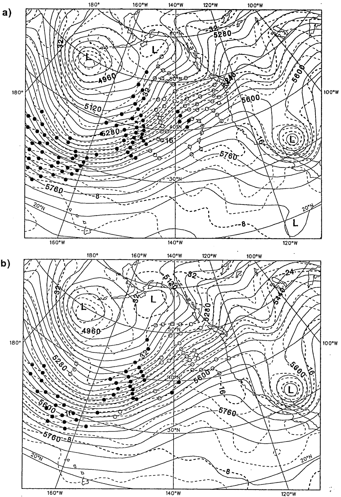
Fig. 4 Analyzed 500 hPa geopotential height (full lines) and temperature (dashed) 31 January 1987, 12 UTC. The markers in the intersections between height contours and temperature contours indicate temperature advection, full circles for cold and open circles for warm air advection. (a) is OPS-July 88 and (b) is NOSATEM.
