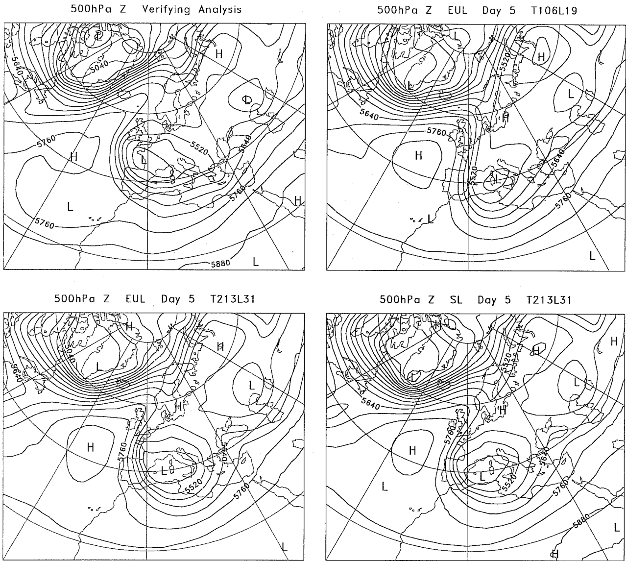
Fig. 5 The analyzed 500hPa height (upper left, contour interval 60m) for 20 April 1990, and day-5 forecasts verifying at this time for:
