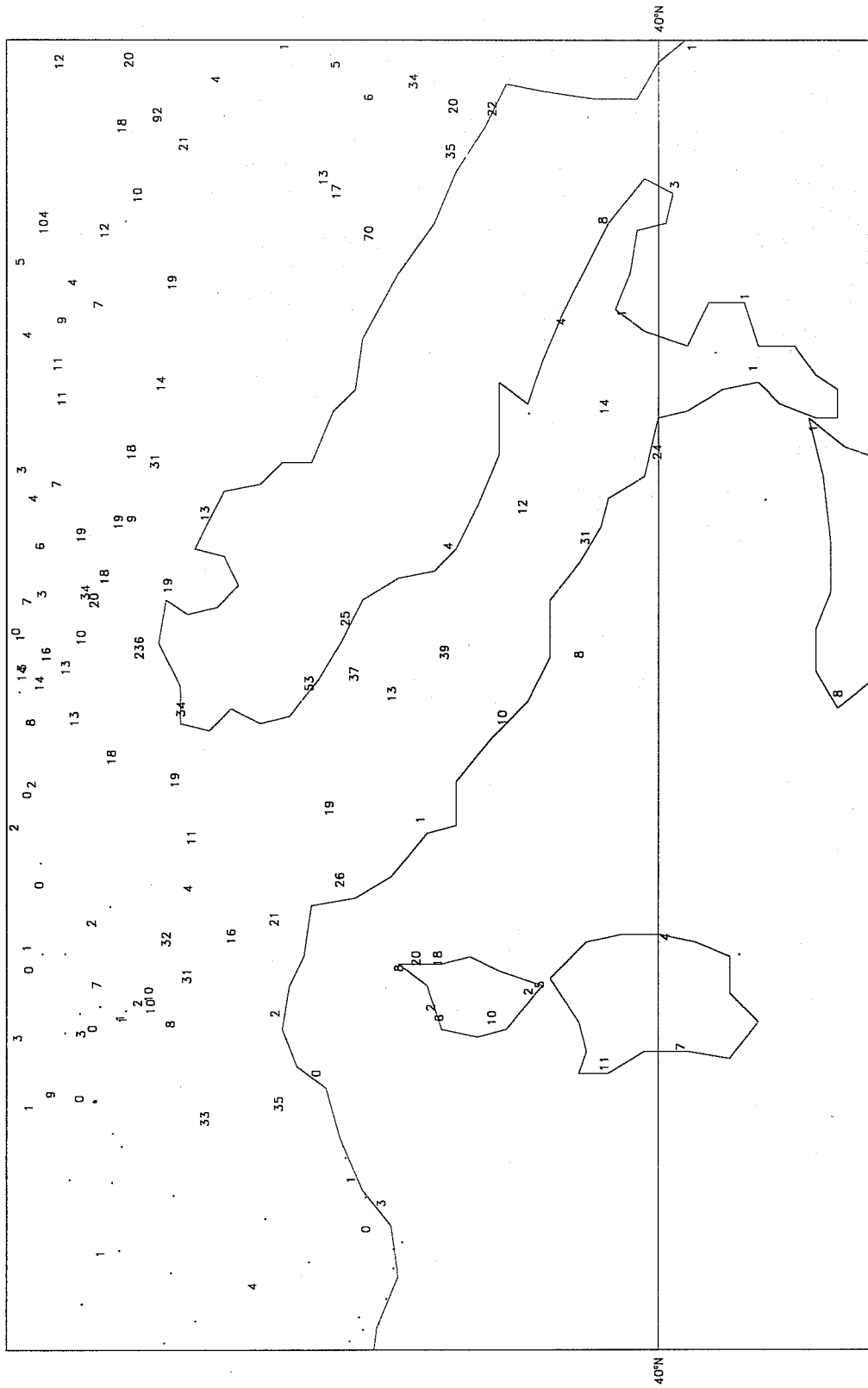
Fig. 11 Observed precipitation (mm) for the period from 12UTC 17 April to 12UTC 18 April 1991.
