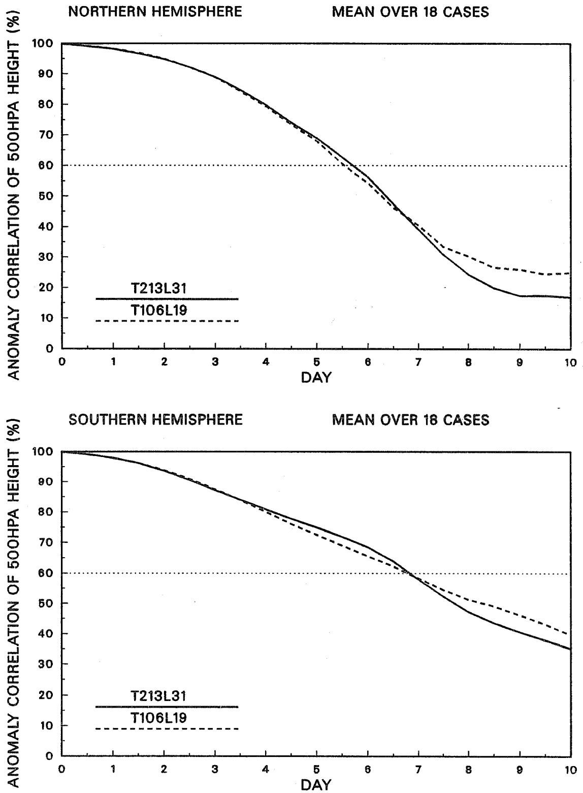
Fig. 21 Mean anomaly correlations of 500hPa height for T213/L31 (solid) and T106/L19 (dashed) for the extratropical northern (upper) and southern (lower) hemispheres, from daily forecasts for the period 11-28 July 1991.
