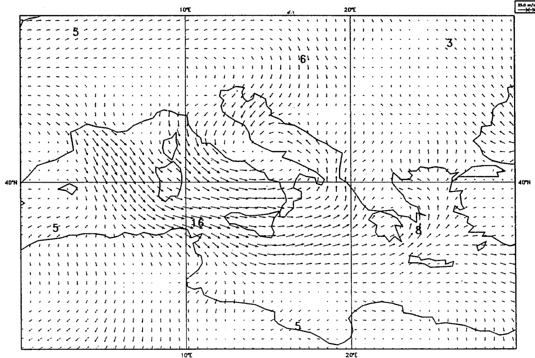
Fig. 6 24-hour forecasts of 10m wind ( \text{ms}^{-1} ) from 15 April 1990, for: Upper: T213/L31, Semi-Lagrangian, \Delta t = 20\text{min} . Lower: T213/L31, Eulerian, \Delta t = 3\text{min} .
