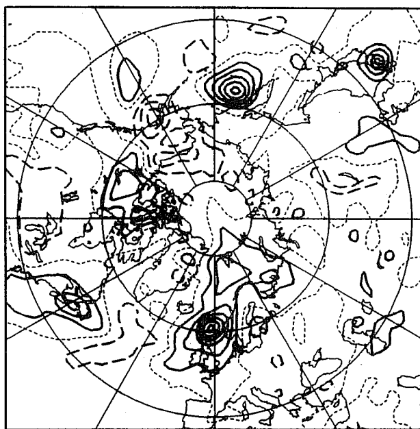
1000hPa Z T106L19-T213L31
