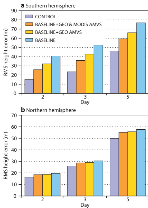
Figure 10 (Above) Impact of MODIS AMVs on 500 hPa geopotential height for (a) southern hemisphere (20°–90°S) and (b) northern hemisphere (20°–90°N).
