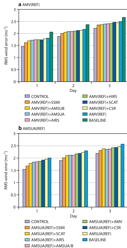
Figure 9 Impact of all sensors on 1000 hPa vector wind for the tropics based on (a) AMV(REF) and (b) AMSUA(REF) .
