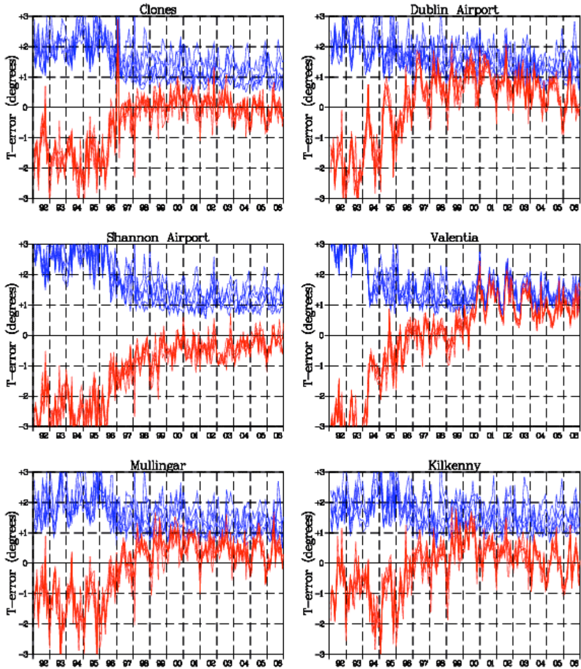
Monthly Scores [Mean/Abs] for Temperature Forecasts Verifying at Midnight
