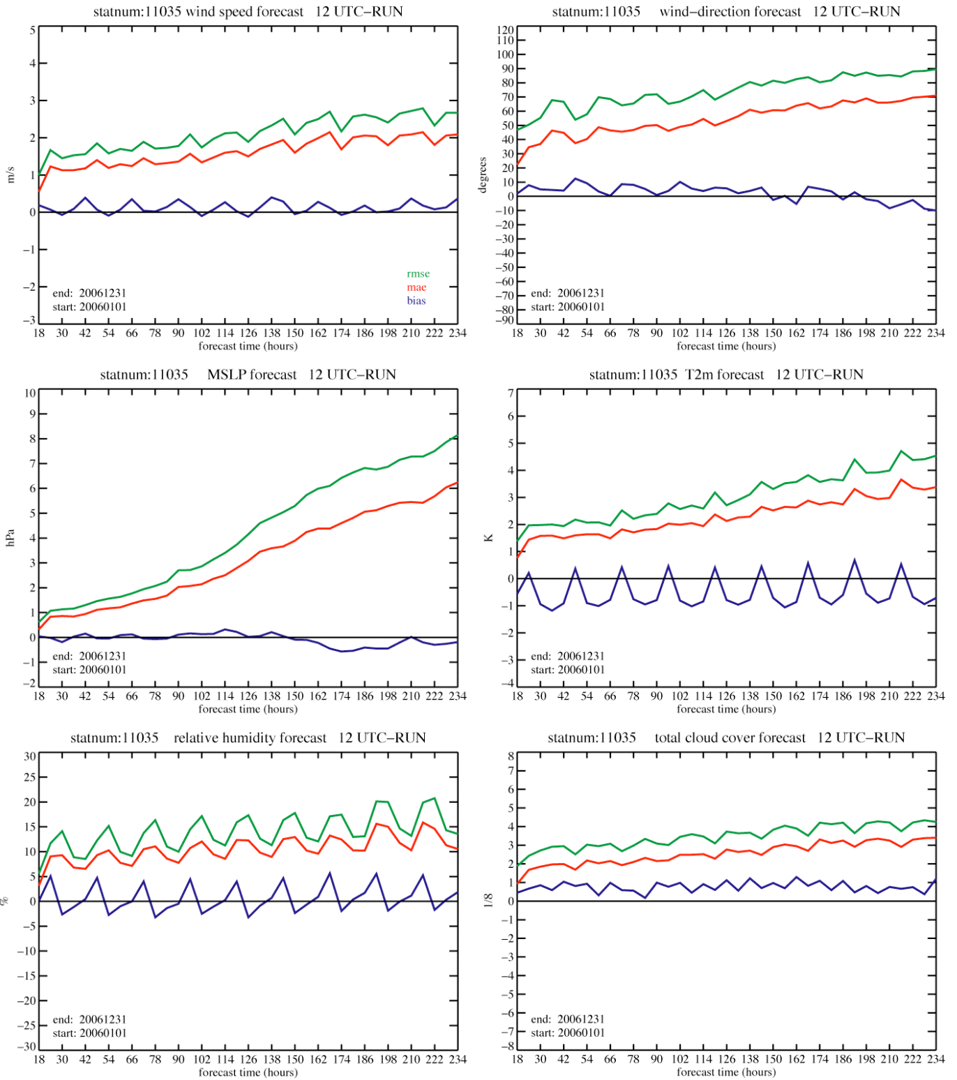
Figs. 6-11 Mean error (bias), mean absolute error (MAE) and RMSE of ECMWF point forecasts of 10m wind speed and direction, msl pressure, total cloudiness, 2m temperature and 2m relative humidity as a function of forecast range for station WIEN in the period Jan-Dec 2006.
