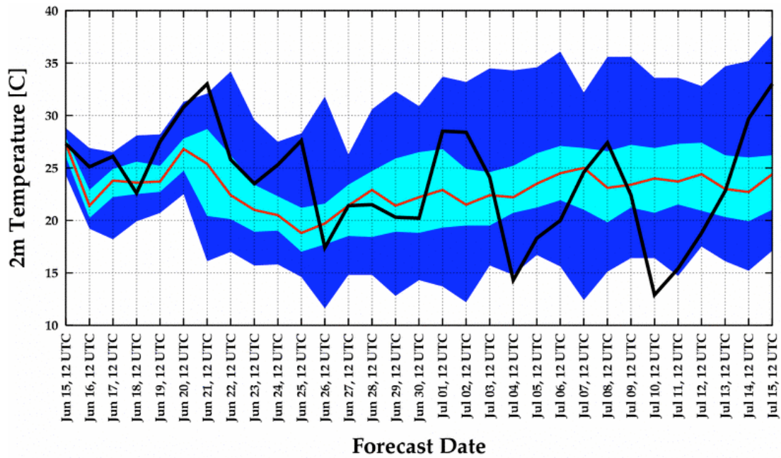
Fig. 13 Ensemble-forecast (blue area+red line) and measured (black line) 2m-temperature for the station Vienna for 12 UTC of ECMWF monthly forecast issued in June.
