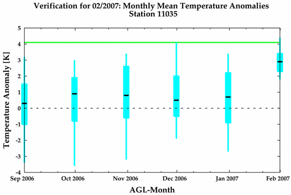
Fig. 12 Comparison of forecasted (bars) and measured (green line) temperature anomalies for the station Vienna. All forecasts valid for February 2007. Abscissa shows the month of the forecast issue.
