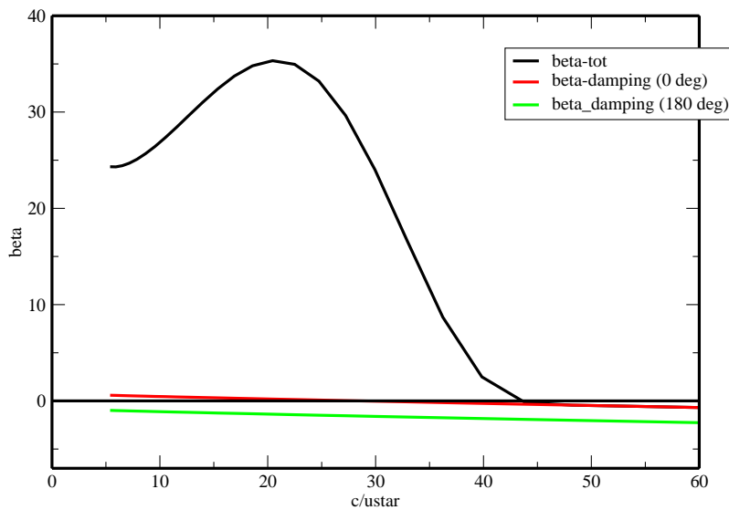
Figure 3.3 The Miles parameter \beta as function of c/u_* for waves propagating in the wind direction. The effect of air turbulence on the growth rate for two different propagation directions is shown as well.
