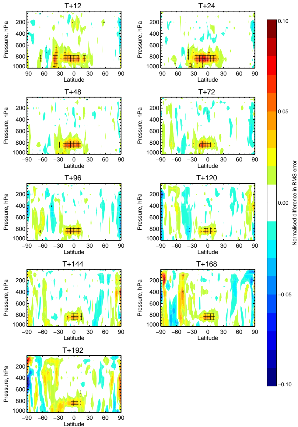
RMS forecast errors in T(amsua-contr), 17-Jan-2011 to 14-Jul-2011, from 61 to 77 samples. Point confidence 99.8% to give multiple-comparison adjusted confidence 95%. Verified against own-analysis.
