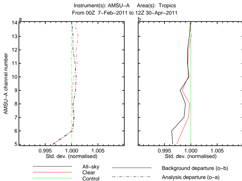
Figure 9: As Fig. 9 but for AMSU-A clear-sky channels
