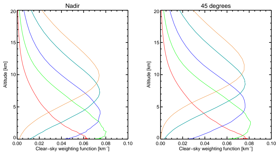
Figure 1: Global average clear-sky weighting functions at nadir (left) and at zenith angle of 45^\circ (right) of AMSU-A channels 3 (red), 4 (green), 5 (dark blue), 6 (light blue) and 7 (orange). Weighting functions are computed as -d\tau(\ln P)/d\ln P where \tau is transmittance and P is pressure. The figure shows the global average of weighting functions computed from a large set of ECMWF atmospheric profiles.
