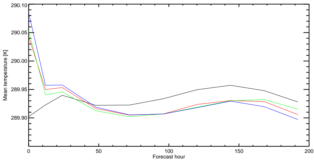
Figure 18: As Fig. 17 but for temperature.
