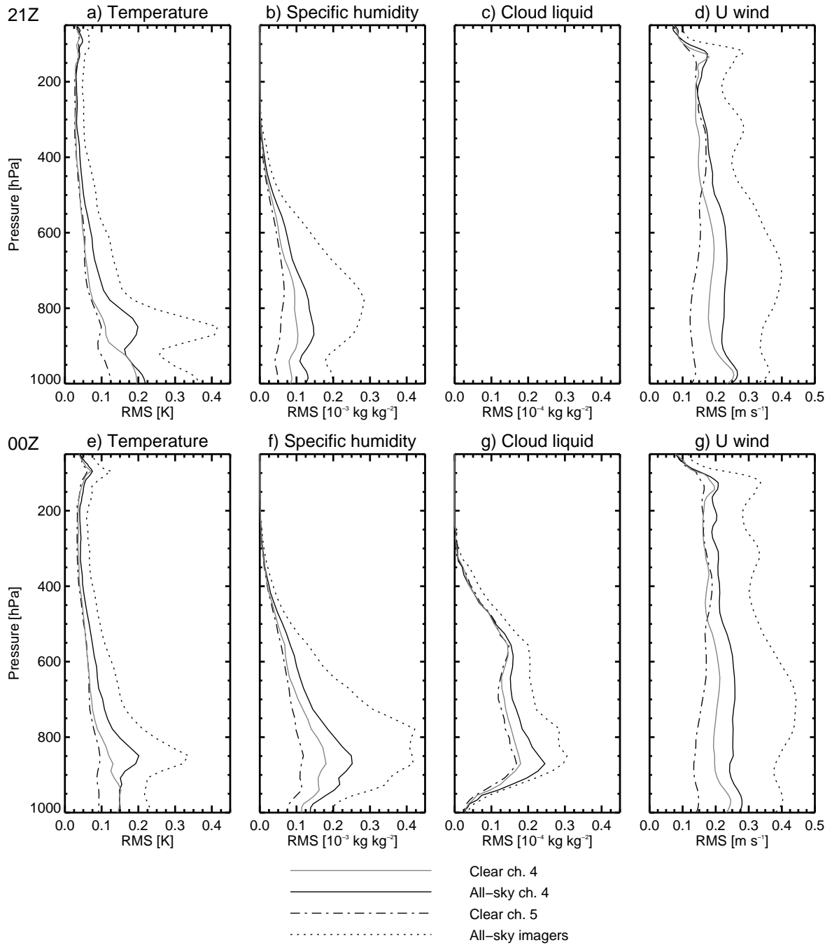
Figure 13: RMS of increments between 40°S and 40°N at the beginning of the assimilation window (a-d) or three hours in (e-h) coming from either clear-sky ch. 4 AMSU-A (grey solid), all-sky ch. 4 AMSU-A (black solid), clear-sky ch.5 (dot-dash) or all-sky microwave imagers (dotted) based on single-cycle experiments with a common FG at 21Z on 14 Feb 2011. There is no cloud liquid water (CLW) control variable as yet, so the 00Z CLW increments are zero.
