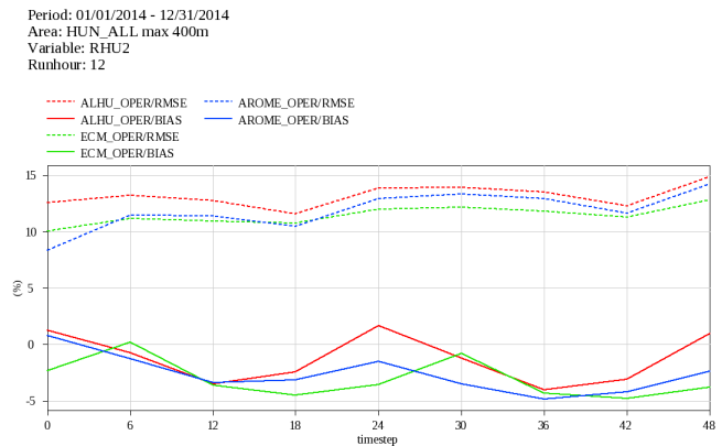
Fig.4 Comparison of BIAS and RMSE values of 2m relative humidity forecasts of the ECMWF HRES (green), ALADIN/HU (red) and AROME (blue) models over Hungary.
