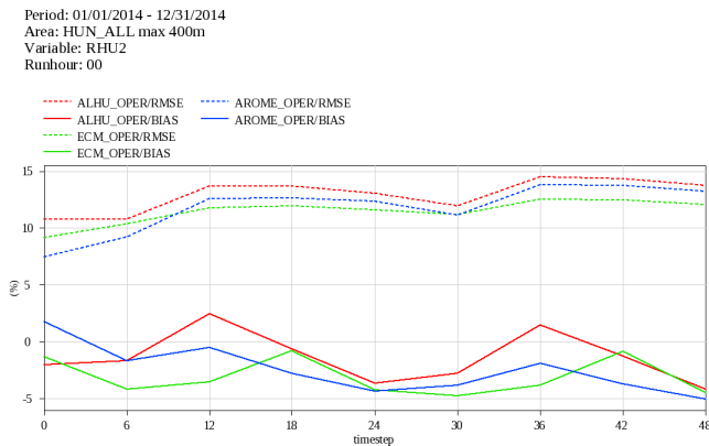
Fig.4 Comparison of BIAS and RMSE values of 2m relative humidity forecasts of the ECMWF HRES (green), ALADIN/HU (red) and AROME (blue) models over Hungary.
