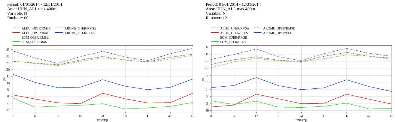
Fig. 6 Comparison of BIAS and RMSE values of total cloudiness forecasts of the ECMWF HRES (green), ALADIN/HU (red) and AROME (blue) models over Hungary
