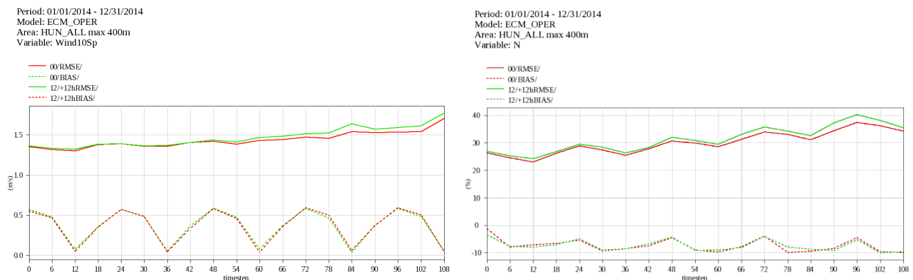
Fig. 2 RMSE and BIAS values of 10m wind speed and total cloudiness forecasts of the ECMWF HRES for Hungary.
