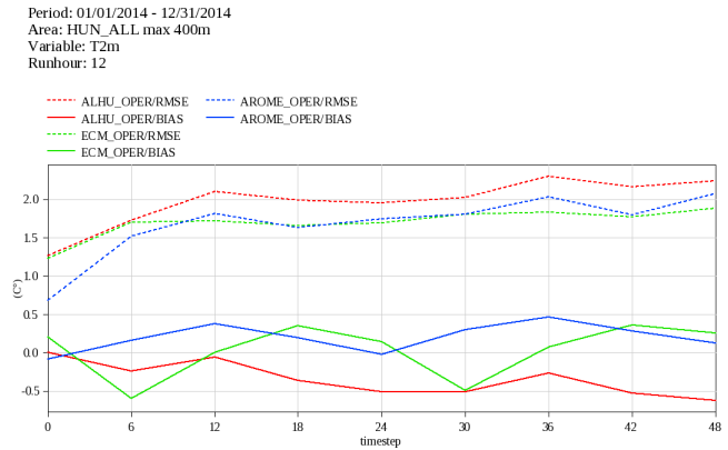
Fig. 3 Comparison of BIAS and RMSE values of 2m temperature forecasts of the ECMWF HRES (green), ALADIN/HU (red) and AROME (blue) models over Hungary.
