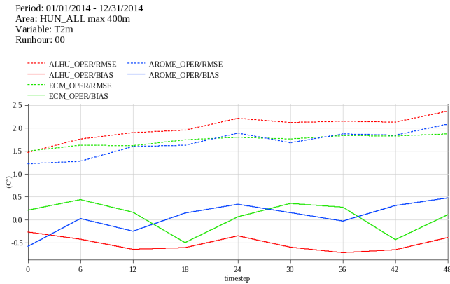
Fig. 3 Comparison of BIAS and RMSE values of 2m temperature forecasts of the ECMWF HRES (green), ALADIN/HU (red) and AROME (blue) models over Hungary.
