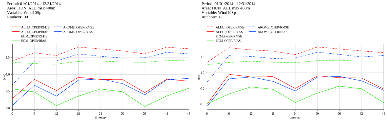
Fig. 5 Comparison of BIAS and RMSE values of wind speed forecasts of the ECMWF HRES (green), ALADIN/HU (red) and AROME (blue) models over Hungary.
