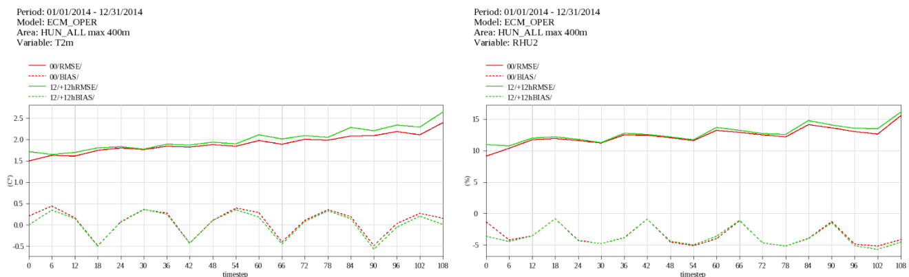
Fig. 1 RMSE and BIAS values of 2m temperature and 2m relative humidity forecasts of the ECMWF HRES for Hungary.
