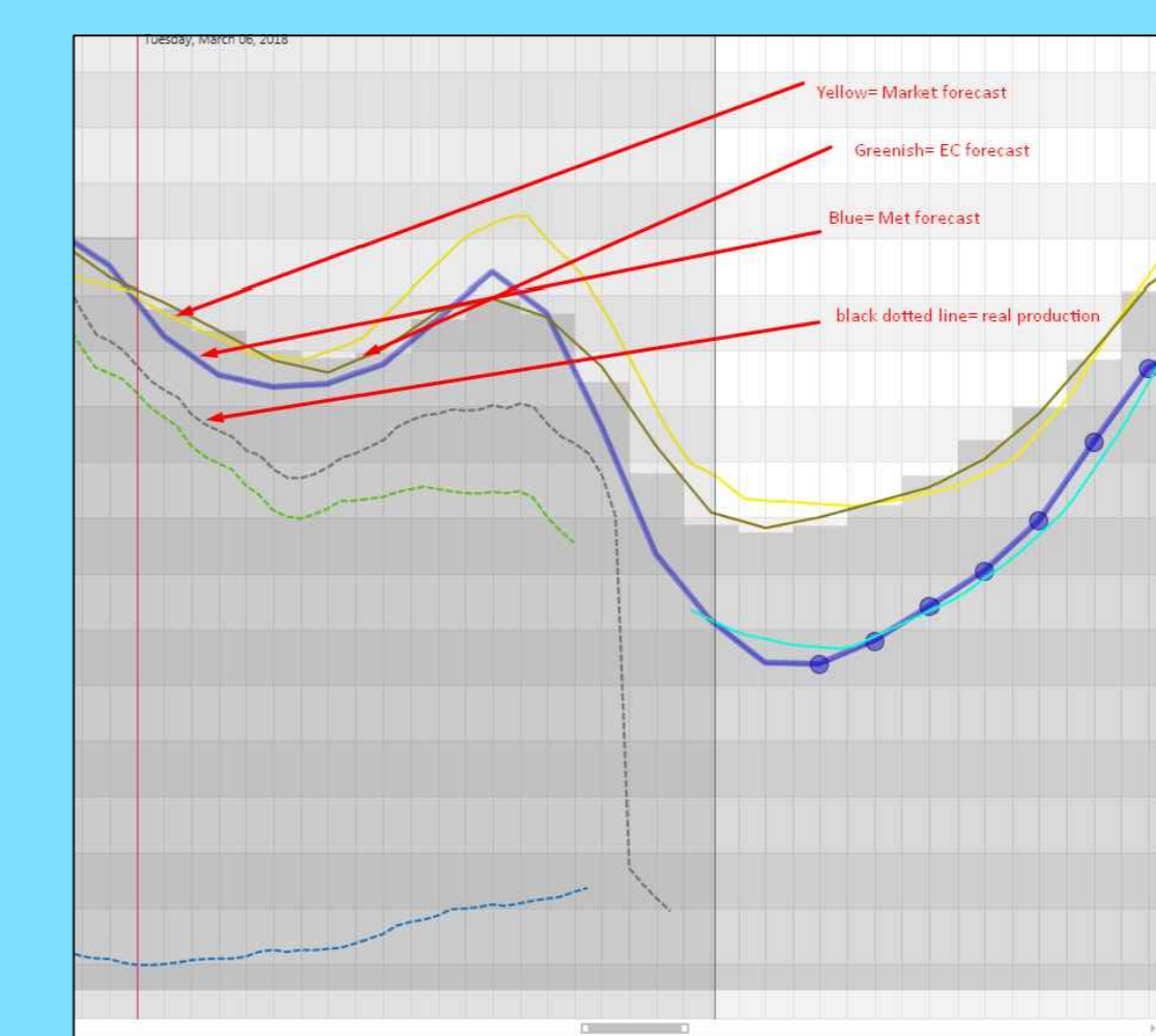
Forecast and real production for the night hours on 06.03.2018
