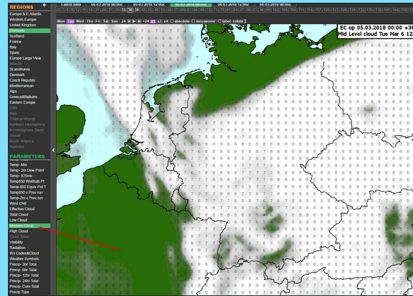
Medium clouds estimation latest run for 06.03.2018
