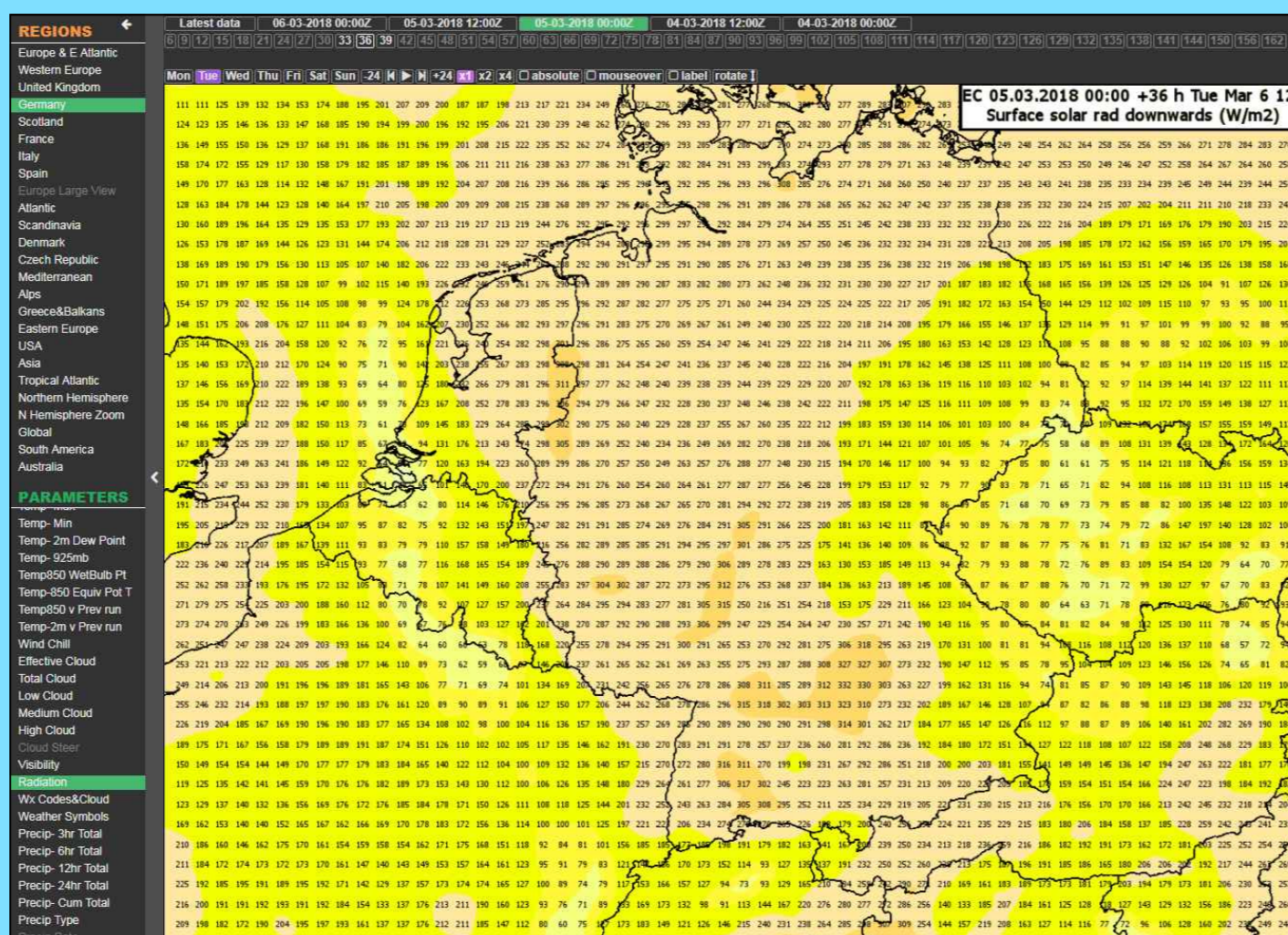
Radiation map on Intraday for 06.03.2018 with 00Z run
